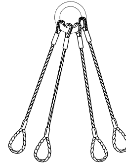
Four leg sling with main ring with thimble at top and plain loops at bottom.
